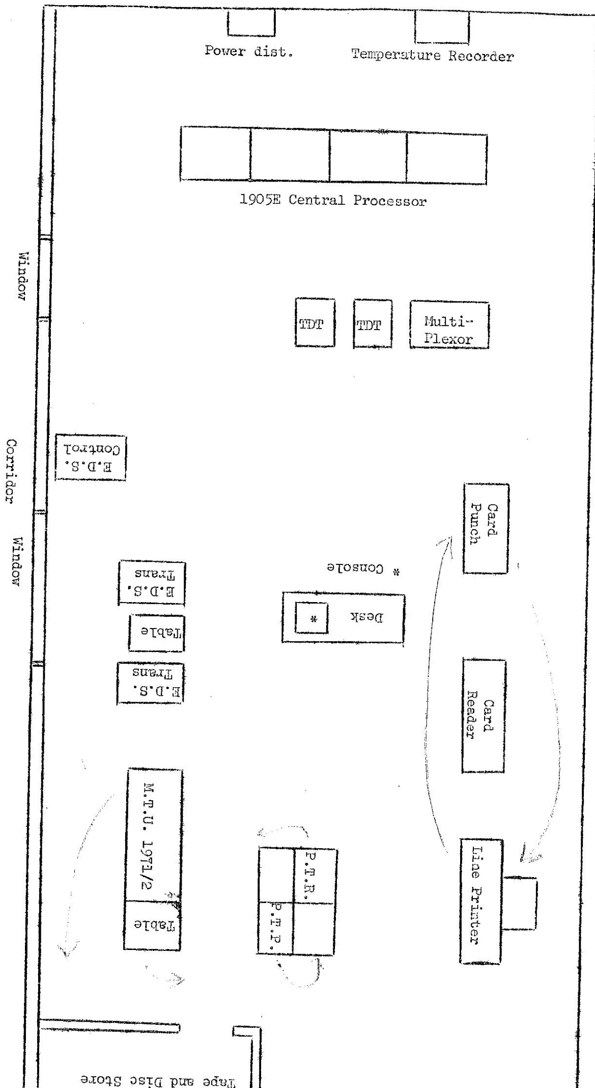
PLAN OF THE MACHINE ROOM
